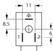
M12 x 1 male connector (5.31T)
