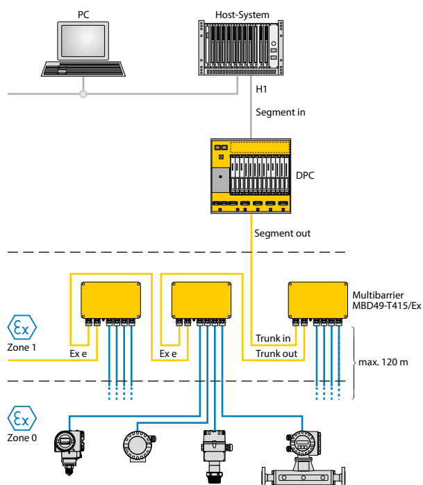
Fig. 3 Topology – FOUNDATION™ in the hazardous area
