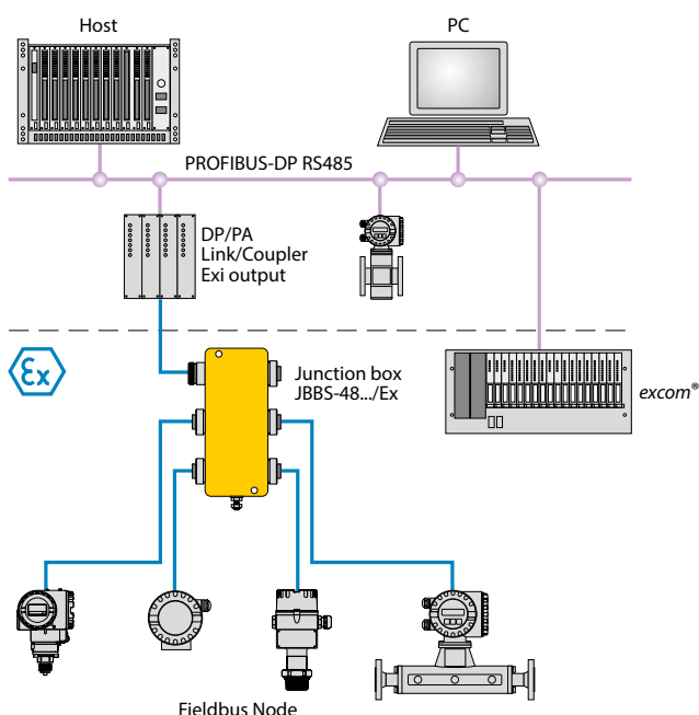
Fig. 3 Topology – PROFIBUS DP in the Ex area with DP/PA coupler (equipped with intrinsically safe outputs)
